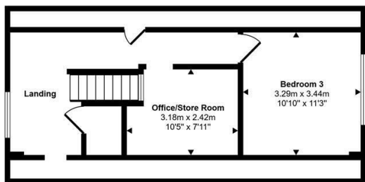
First Floor Approx 46 sq m / 493 sq ft
